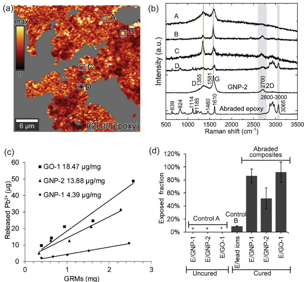
Fig. 3 Qualitative and quantitative detection of GRMs released from abrasion. Raman spectroscopy mapping of the abraded particles from E/GNP-2 showing (a) map of the ratio of the intensity of the 2D band (center at 2700 cm -1 ) as a marker of GNP-2 to the intensity of an epoxy related Raman band (center at 3065 cm -1 ). The compared Raman bands are indicated in (b) by gray areas. (b) Representative Raman spectra from different regions in the mapping area as compared to the reference GNP-2 and abraded neat epoxy. Red lines are a guide to the eye indicating the GNP-2 related Raman bands. (c) Pb 2+ release capacity of GNP-1, GNP-2, and GO-1 from one representative example of each material. (d) Bar chart of the release fraction of Pb 2+ from the control samples and the exposed fraction of GRMs from three epoxy/GRM composites. Three measurements were performed for each sample. The average mean values are reported with the standard deviations. The concentration of Pb 2+ in control A (uncured samples) was below the detection limit of 0.1 mg L -1 , which is marked by *.
